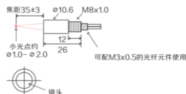
EFG-6HA (35mm处小光斑)
