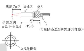
EFG-2HA (7mm处小光斑)
